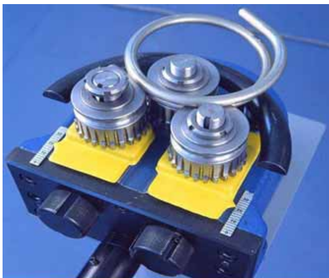
AS 20-1 Biegemaschine
